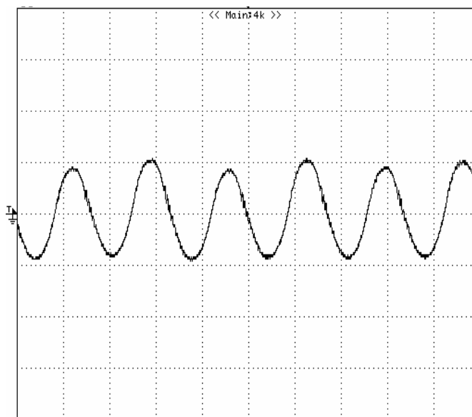
Figure 11: Input Terminal Ripple Current, i_c , at full rated output current and nominal input voltage with 12\mu H source impedance and 33\mu F electrolytic capacitor (500 mA/div, 2\mu s /div).
