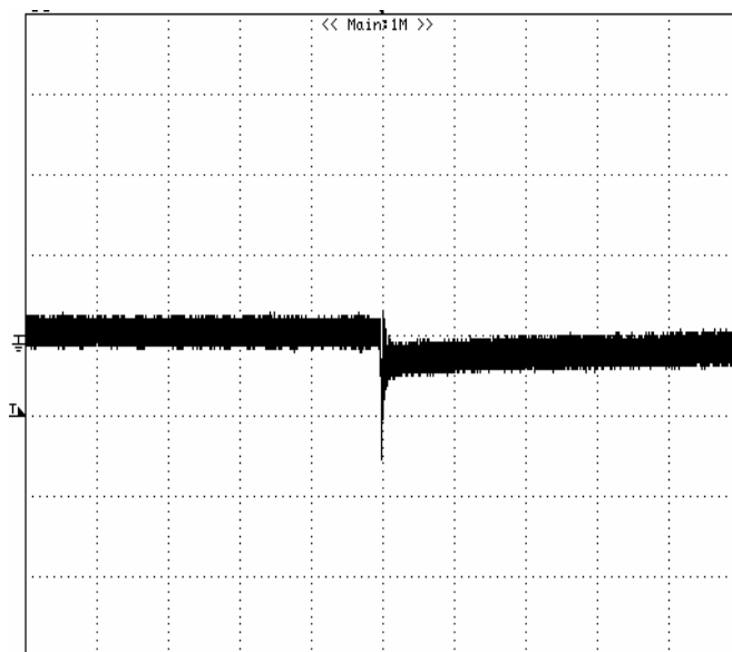
Figure 9: Output voltage response to step-change in load current (50%-75% of I_o , max; di/dt = 0.1A/\mu s ). Load cap: 10\mu F , tantalum capacitor and 1\mu F ceramic capacitor. Trace: V_{out} (200mV/div), Scope measurement should be made using a BNC cable (length shorter than 20 inches). Position the load between 51 mm to 76 mm (2 inches to 3 inches) from the module.
