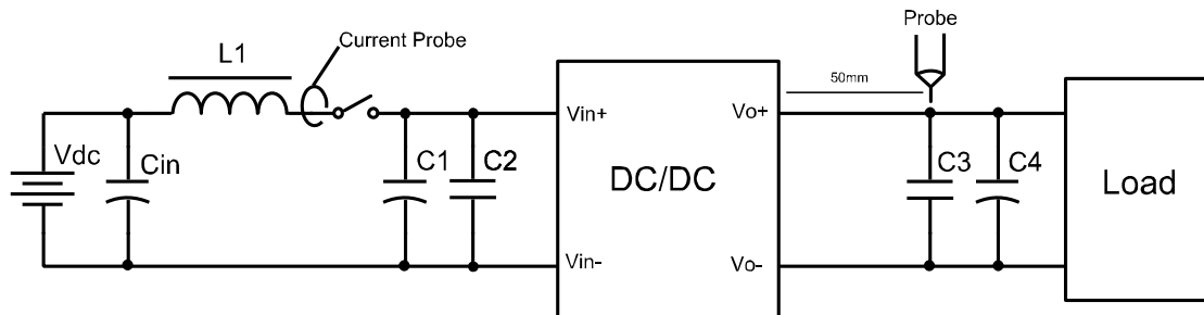
Figure 26 Input ripple & inrush current output ripple & noise test configuration
