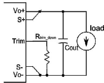
Figure 25 Trim down
