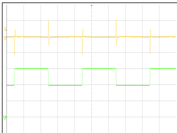
Figure 7: AVO75B-36S3V3 Transient Response (2mS/div) 50%~75%~50% load change, 0.1A/uS slew rate, Ch 1: Vo (50mV/div) Ch 2: Io (5A/div)
