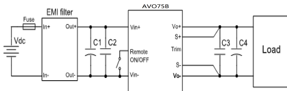
Figure 21 Typical application
