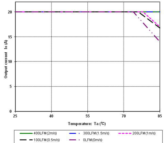
Figure 14 Output power derating, 48V in
