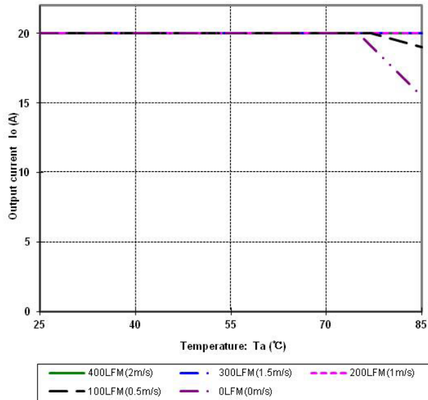
Figure 13 Output power derating, 24V in ,
