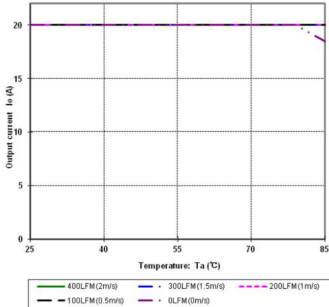
Figure 18 Output power derating, 24V in ,
