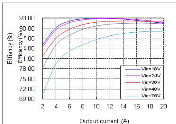
Figure 9: AVO75B-36S3V3 Efficiency Curves @ 25 °C
