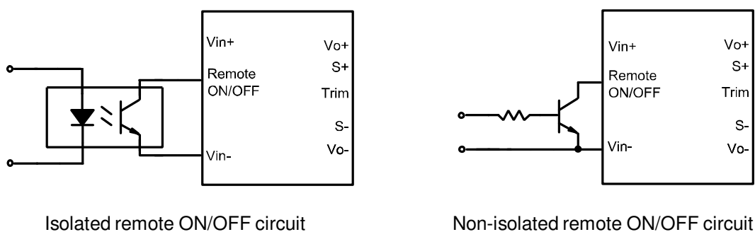
Figure 23 External Remote ON/OFF circuit
