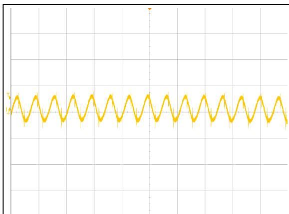
Figure 1: AVO75B-36S3V3 Input Reflected Ripple Current Waveform
