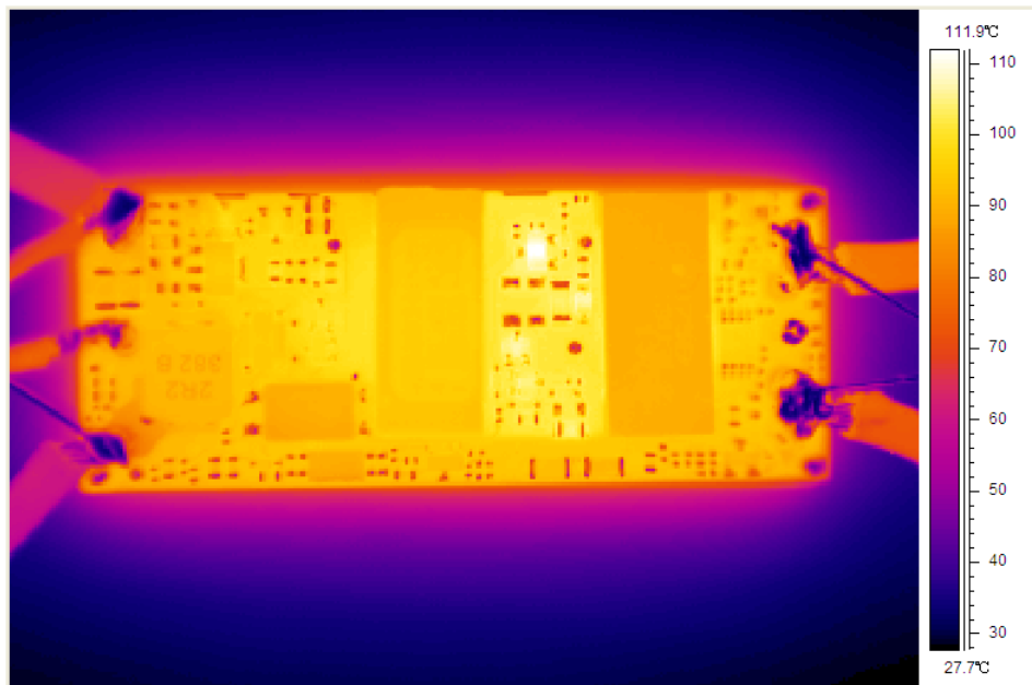
Figure 20 Thermal image, 36V in , 3.3V o , full load, room temperature, 100LFM (air flowing from pin 3 to pin 1)
