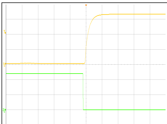
Figure 5: AVO75B-36S3V3 Remote ON Waveform (100mS/div)
