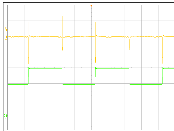
Figure 8: AVO75B-36S3V3 Transient Response (2mS/div) 50%~75%~50% load change, 1A/uS slew rate Ch 1: Vo (50mV/div) Ch 2: Io (5A/div)
