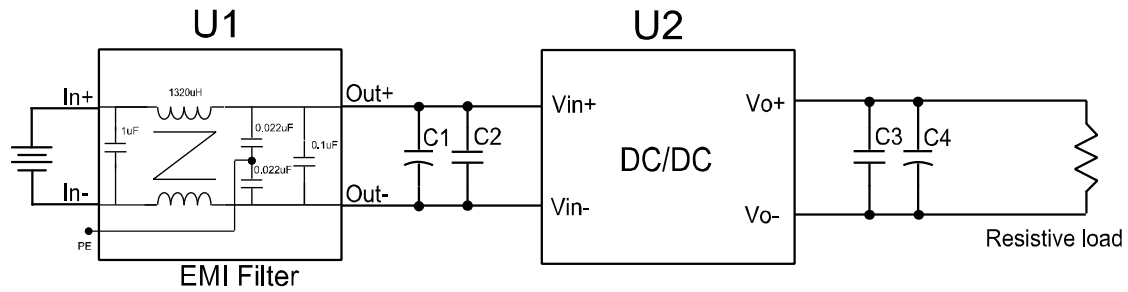
Figure 27 EMC test configuration
