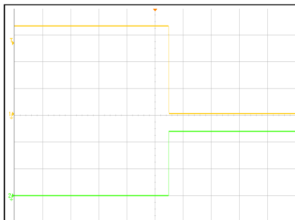
Figure 6: AVO75B-36S3V3 Remote OFF Waveform (50mS/div)
