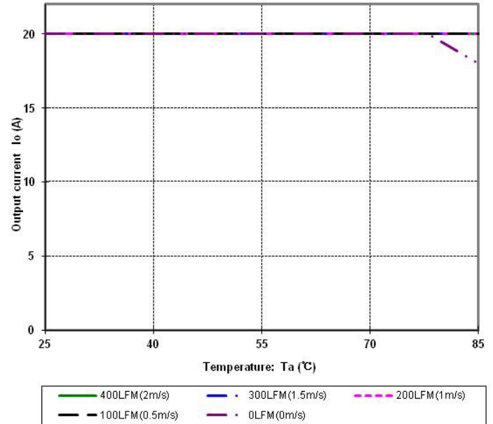
Figure 19 Output power derating, 48V in
