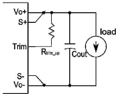
Figure 24 Trim up
