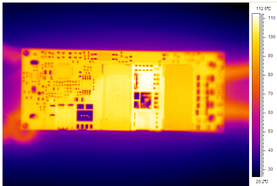
Figure 15 Thermal image, 36V in , 3.3V o , full load, room temperature, 100LFM (air flowing from pin 3 to pin 1)
