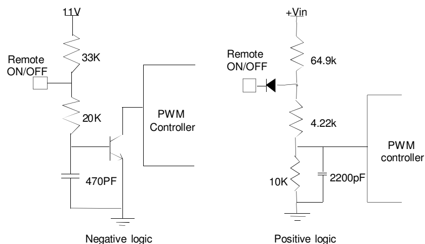
Figure 22 Remote ON/OFF internal diagram
