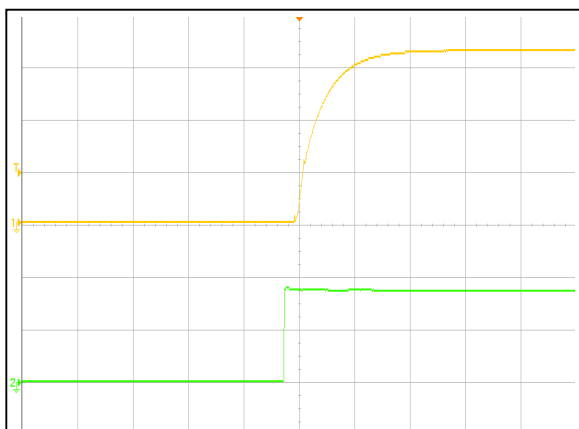
Figure 3: AVO75B-36S3V3 Output Voltage Startup Characteristic (50mS/div)
