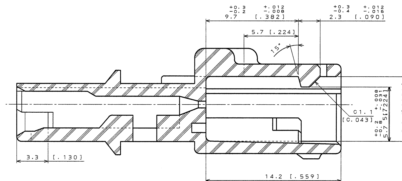
SECTION A-A (SCALE 5/1)
