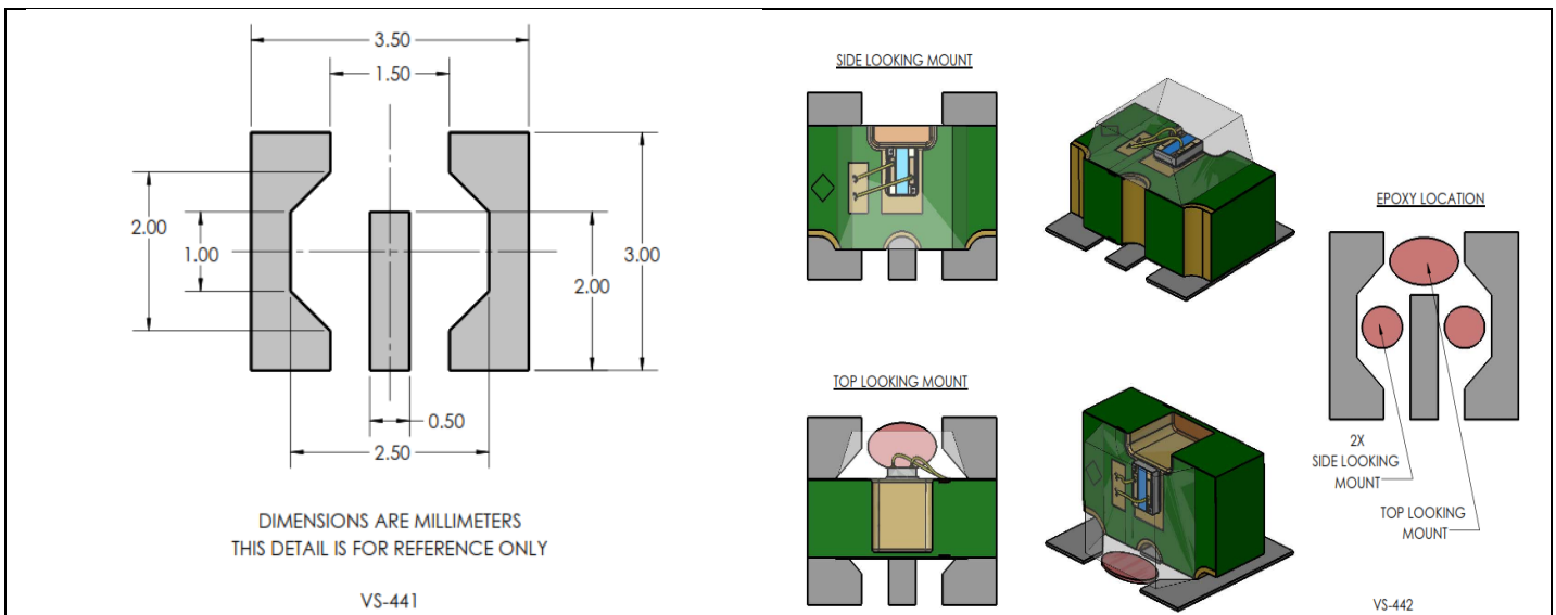
Figure 7: Proposed Soldering Pad Pattern & Dimensions, Top and Side Looking Orientation on Main Board
