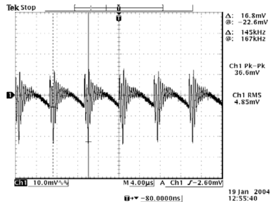
20 Vdc input, 1.5 Vdc output
