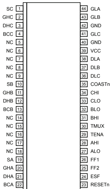
Pin-out Diagram
