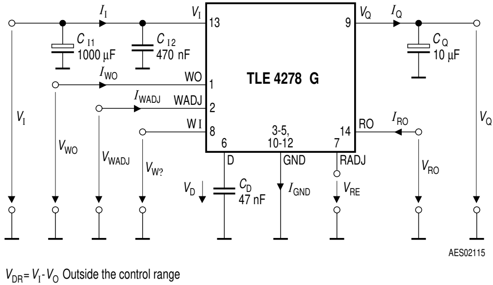
Figure 3 Test Circuit
