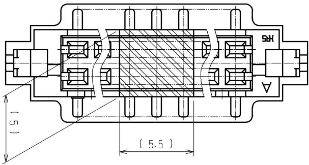
POSITION IN WHICH HEAT-RESISTANCE TAPE IS PUT
