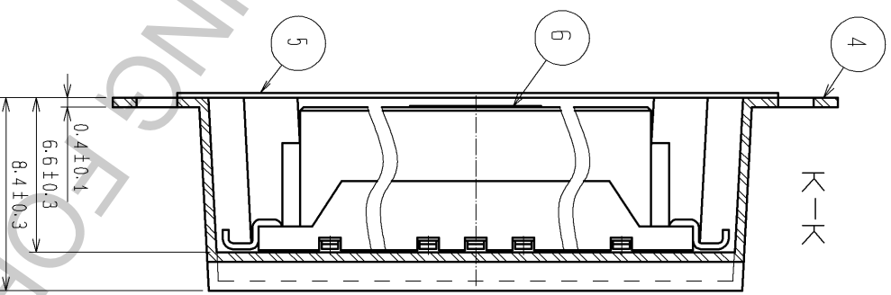
POSITION IN WHICH HEAT-RESISTANCE TAPE IS PUT
