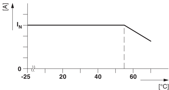
Figure 10 Temperature-dependent derating
