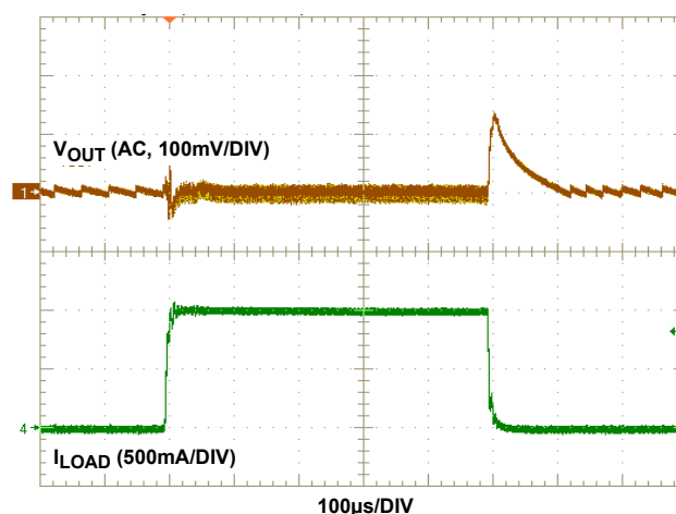
FIGURE 17. 0A TO 1A LOAD TRANSIENT ( V_{IN} = 3.6\text{V} , V_{OUT} = 3.3\text{V} )
