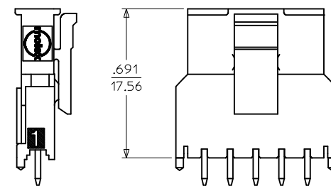
MATED MICRO FIT CONNECTORS
