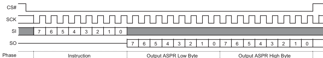
Figure 9.53 ASPRD Command
