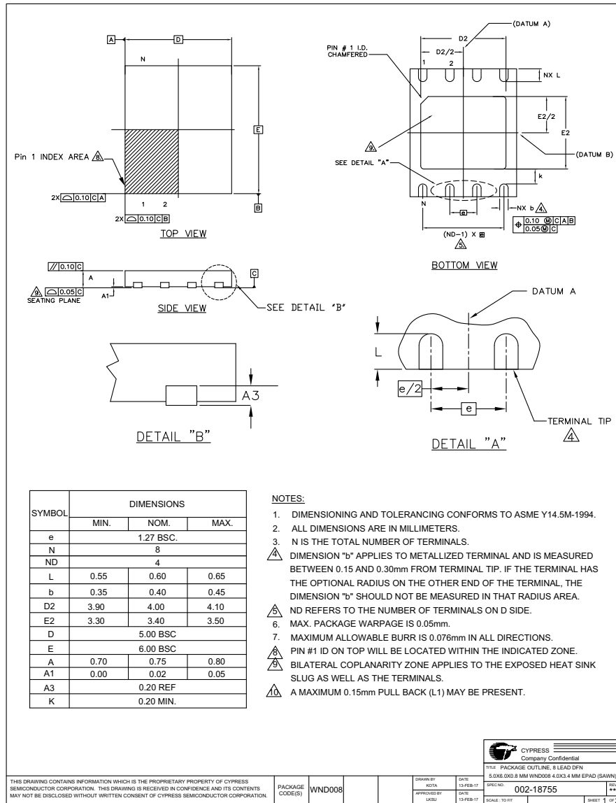
Figure 6.6 WSON 8-Contact 6x5 mm Leadless (WND008)
