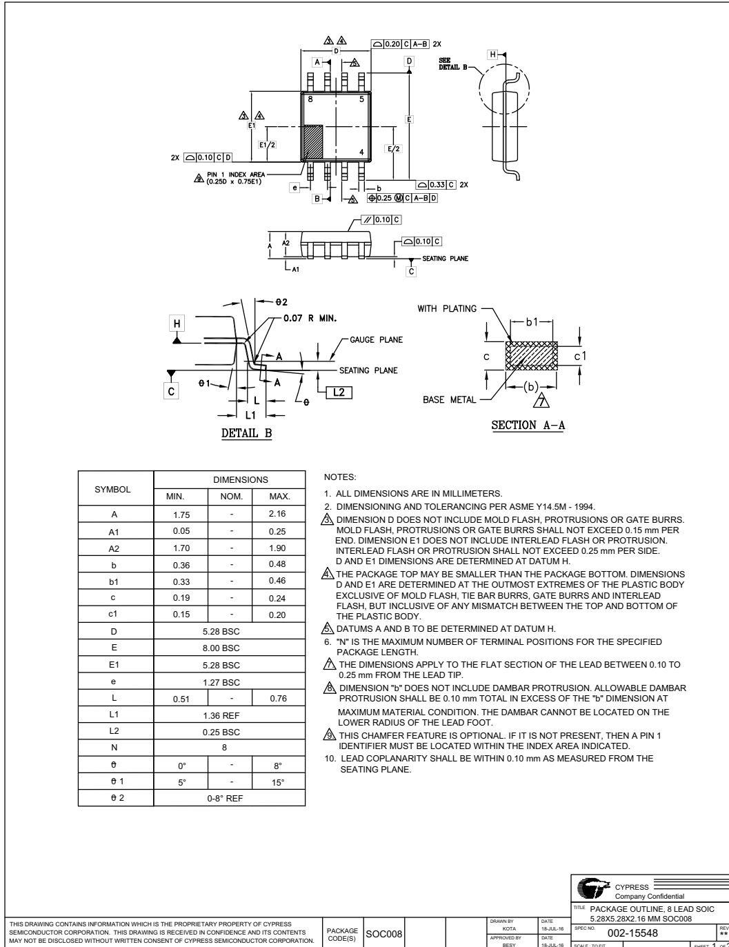
Figure 6.5 SOIC 8-Lead, 208 mil Body Width (SOC008)
