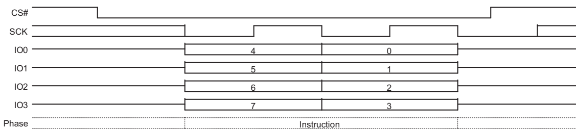
Figure 9.16 Write Disable (WRDI) Command Sequence QPI Mode
