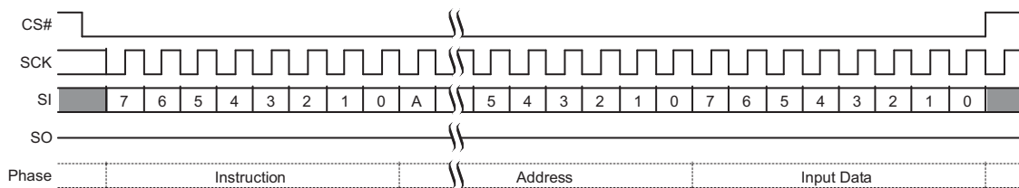
Figure 9.57 DYBWR Command Sequence
