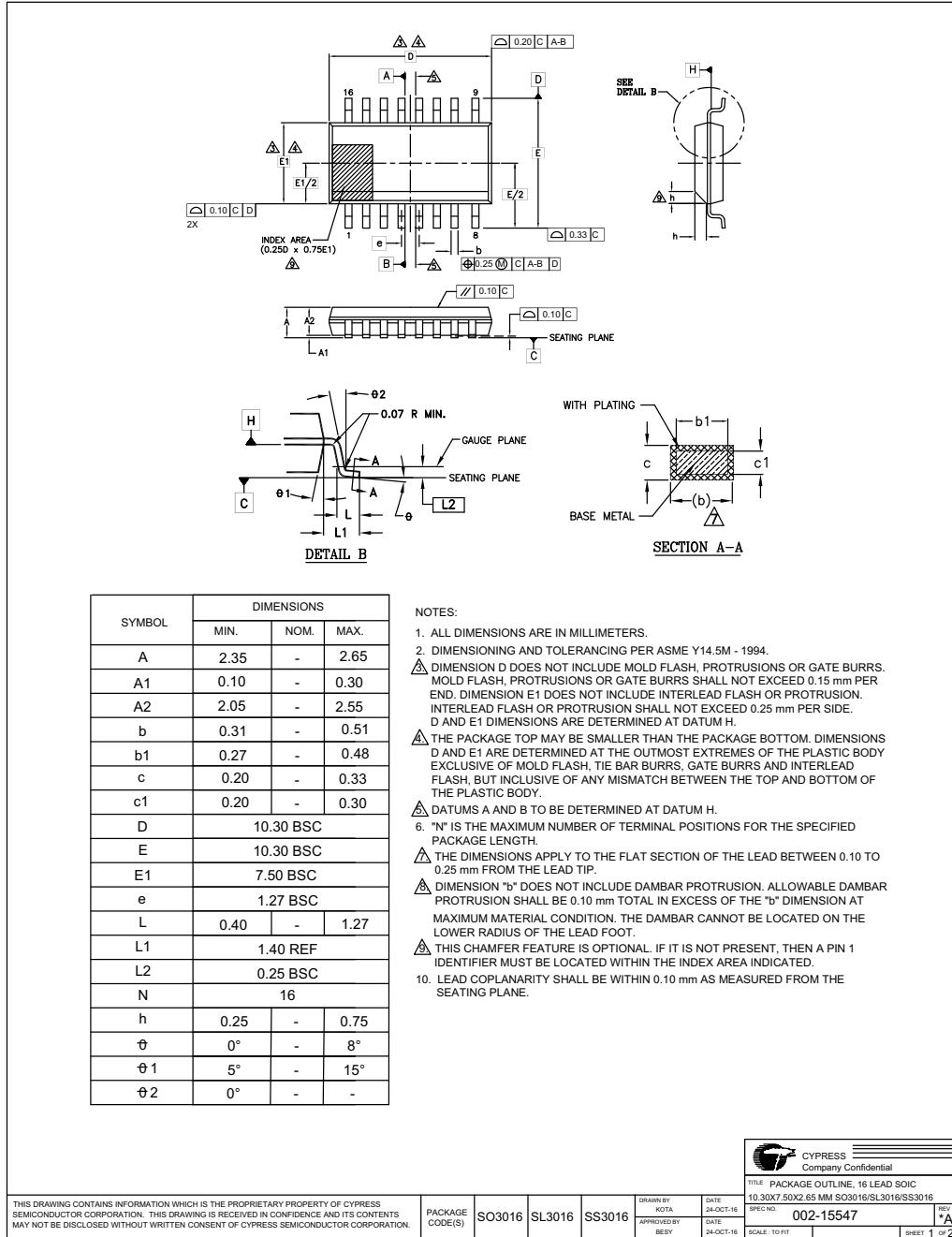
Figure 6.2 SOIC 16-Lead, 300-mil Body Width (SO3016)
