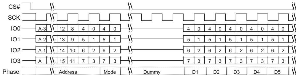
Figure 9.36 Continuous DDR Quad I/O Read Subsequent Access (EDh or EEh)
