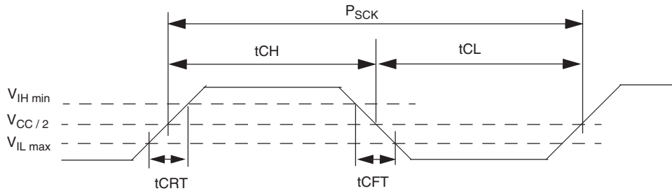
Figure 5.9 Clock Timing
