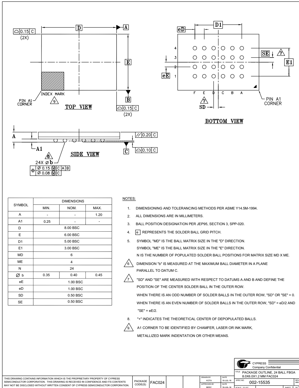
Figure 6.11 Ball Grid Array 24-Ball 6 x 8 mm (FAC024)
