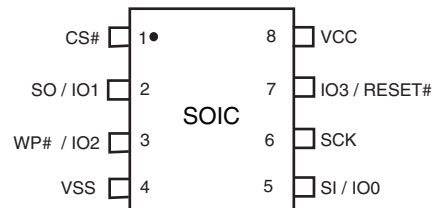
Figure 6.3 8-Pin Plastic Small Outline Package (SOIC8)
