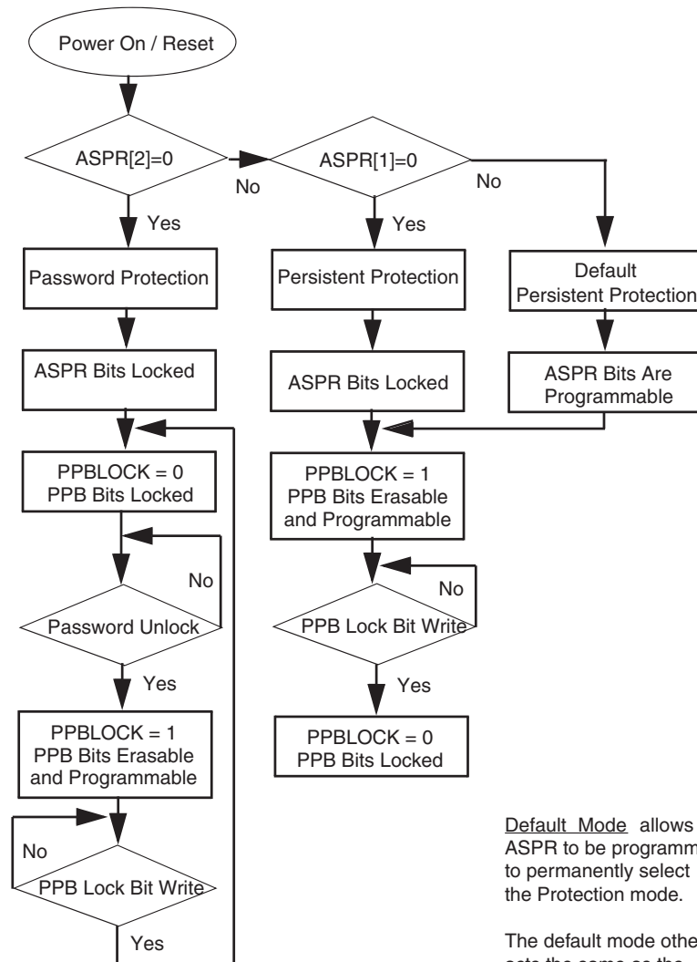
Figure 8.2 Advanced Sector Protection Overview
