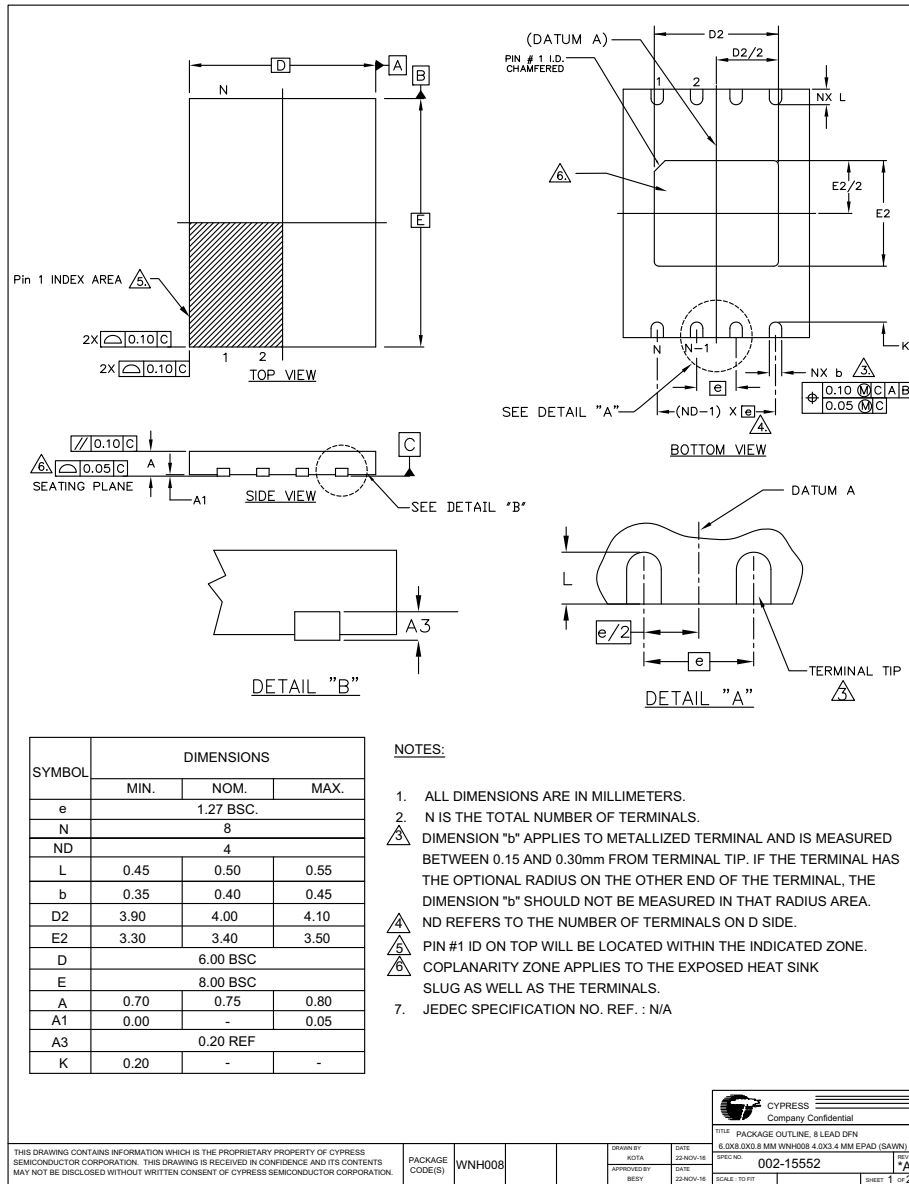
Figure 6.7 WSON 8-Contact 6x8 mm Leadless (WNH008)
