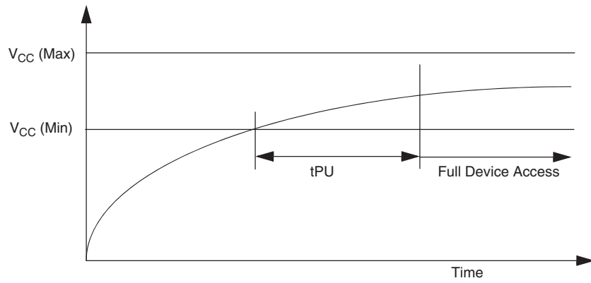
Figure 4.3 Power-Up
