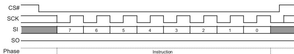
Figure 3.3 Stand Alone Instruction Command
