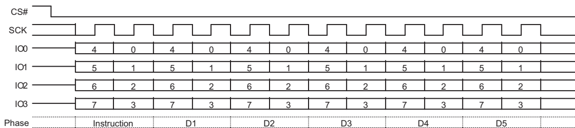
Figure 9.2 Read Identification (RDID) QPI Mode Command
