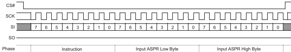
Figure 9.54 ASPP Command
