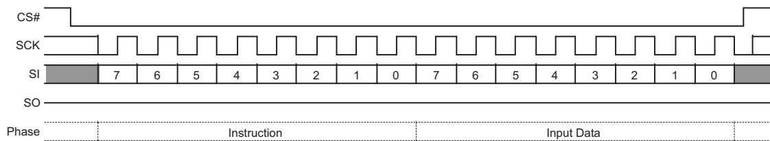
Figure 9.22 Write VDLR (WVDLR) Command Sequence
