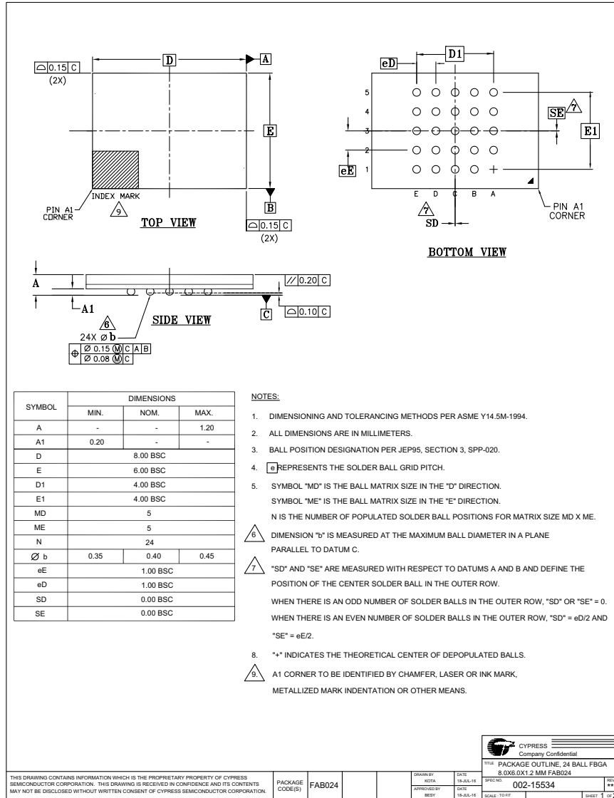
Figure 6.9 Ball Grid Array 24-Ball 6x8 mm (FAB024)
