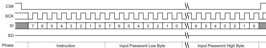
Figure 9.65 Password Program Command Sequence
