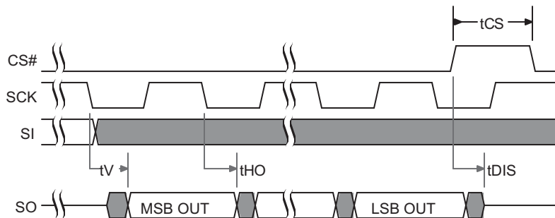
Figure 5.11 SPI Single Bit Output Timing
