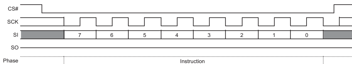
Figure 9.44 Bulk Erase Command Sequence
