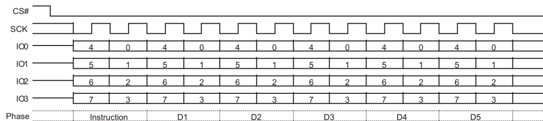
Figure 9.3 Read Quad Identification (RDQID) Command Sequence
