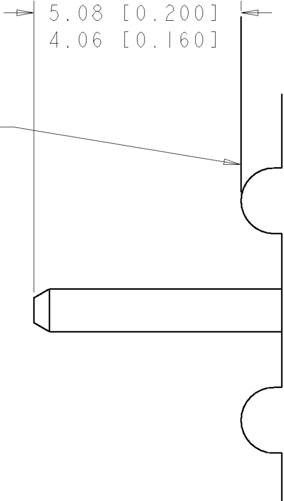
6. SOLDER TAIL DETAIL SCALE 10 : 1
