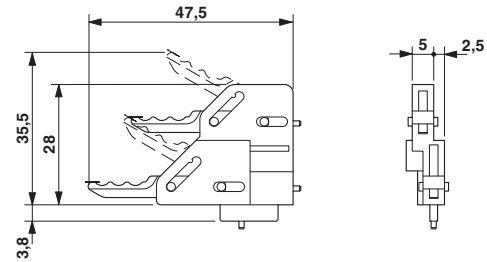
Dimensioned drawing
