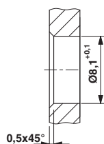
Dimensional drawing
