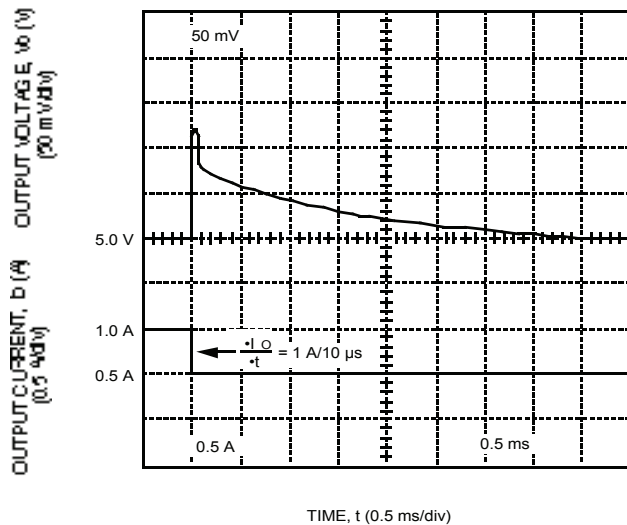
Figure 4. CC025 Dual-Output-Series Typical 5 V Output Voltage Response to a Step Load Change from 50% to 25% of I_{o, \text{max}} at V_i = V_{i, \text{nom}} and T_c = 25^\circ\text{C}
