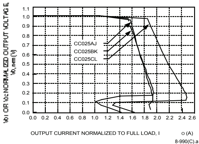
Figure 2. CC025 Dual-Output-Series Normalized Output Current vs. Normalized Output Voltage at V_i = 28\text{ V} and T_c = 25^\circ\text{C}
