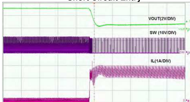
Short Circuit Entry
