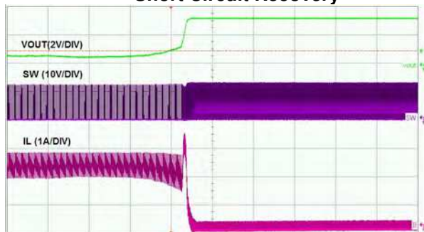
Short Circuit Recovery
