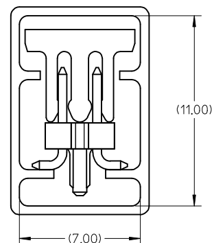
PART WITH CAP IN TUBE (PLS REFER TO PK SPEC: PK-89990-476)
