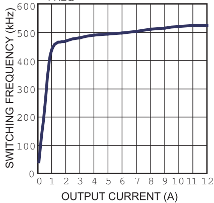
Switching Frequency vs. Output Current
