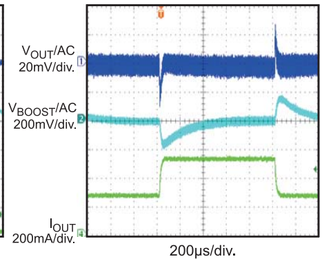
Load Transient
