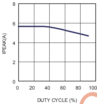
Current Limit vs. Duty Cycle
