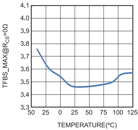
TFBS_MAX@R CS =0Ω vs. Temperature
