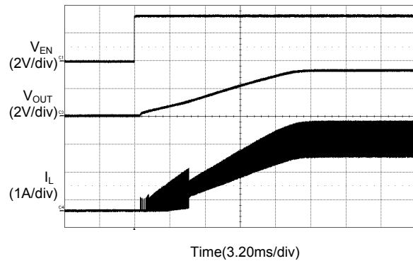
Figure 11. Power On from EN ( I_{OUT}=2.5A )
