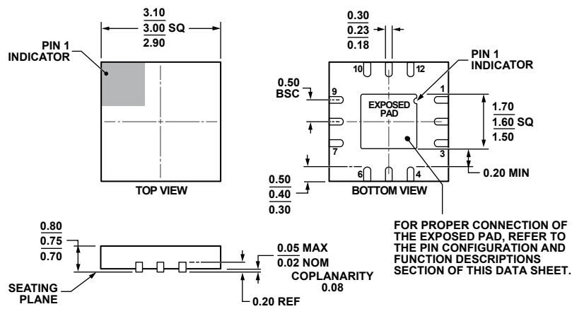
COMPLIANT TO JEDEC STANDARDS MO-229-WEED-4. Figure 16. 12-Lead Lead Frame Chip Scale Package [LFCSP_WQ] 3 mm × 3 mm Body, Very Very Thin Quad (CP-12-6) Dimensions shown in millimeters
