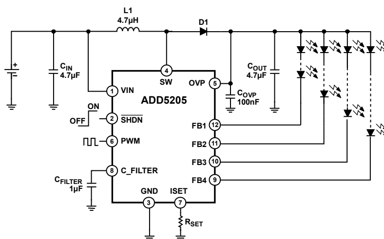
Figure 15. Typical Application Circuit
