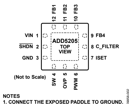
Figure 3. Pin Configuration
