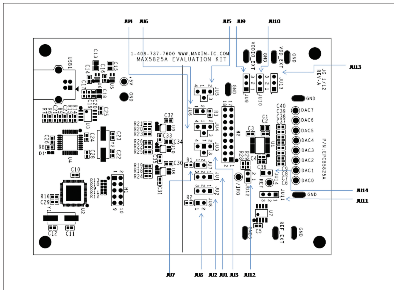
Figure 6. Jumper Callouts
