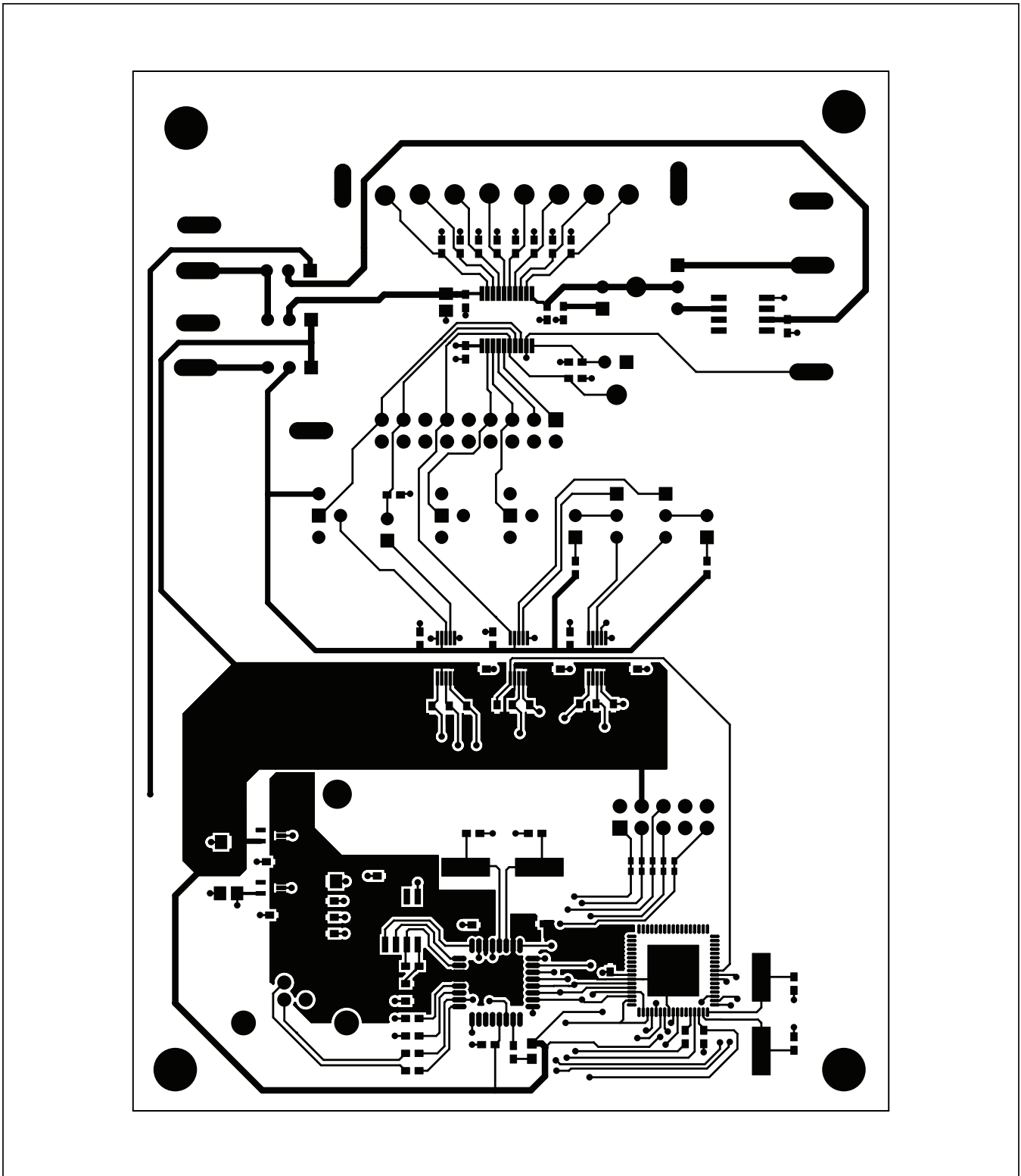
Figure 9. MAX5825A EV Kit PCB Layout—Component Side
