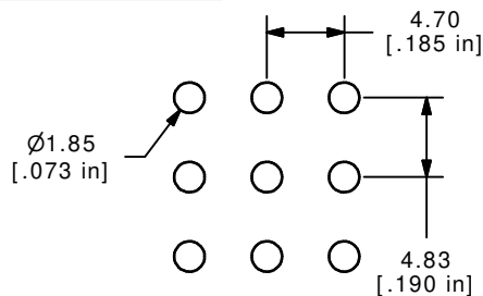
P.C. MOUNTING
