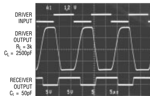
Output Waveforms
