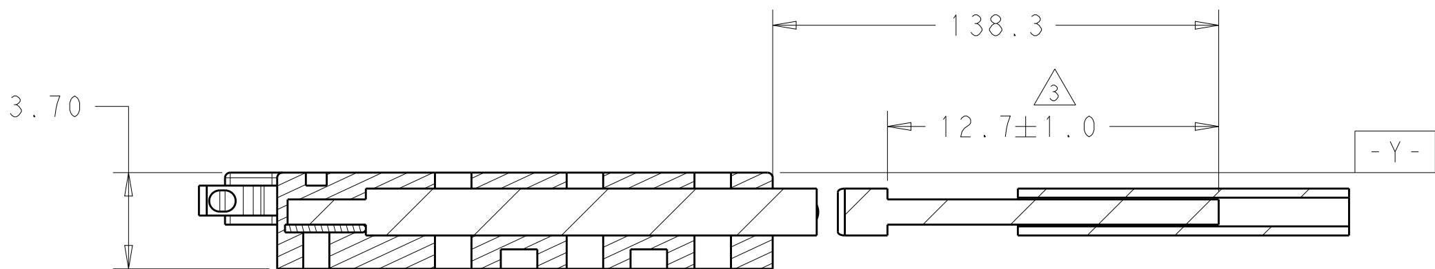
SECTION B-B
