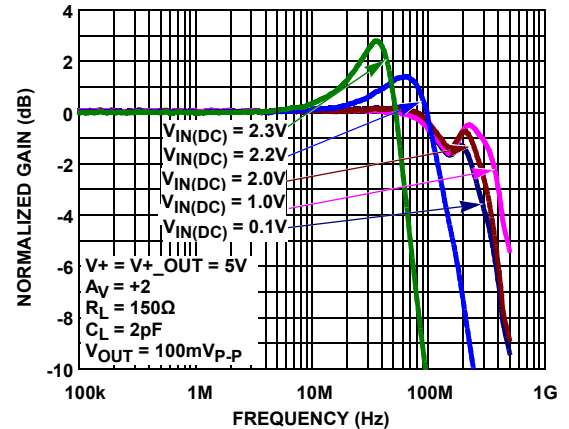
FIGURE 4. GAIN vs FREQUENCY FOR VARIOUS DC INPUT VOLTAGES
