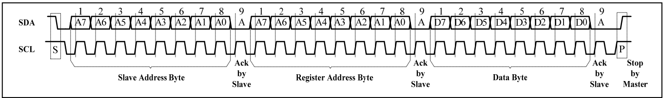
Figure 4 Writing to IS31FL3235A (Typical)
