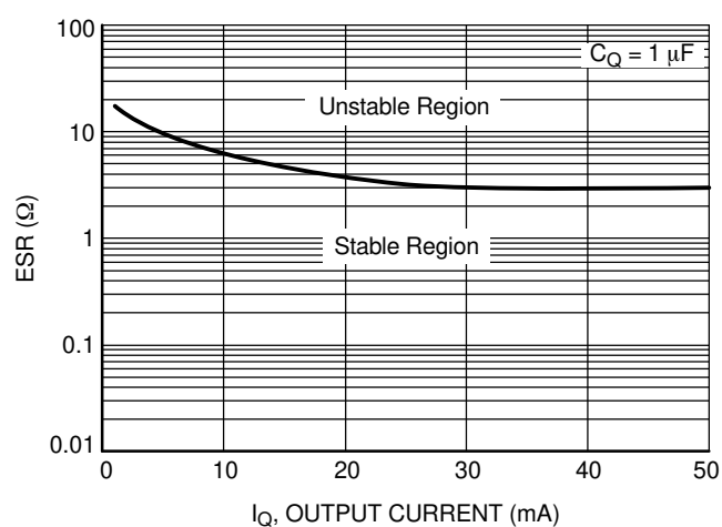
Figure 8. Output Capacitor Series Resistor ESR vs. Output Current I_{out}
