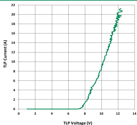
SD05 Transmission Line Pulsing(TLP) Plot
