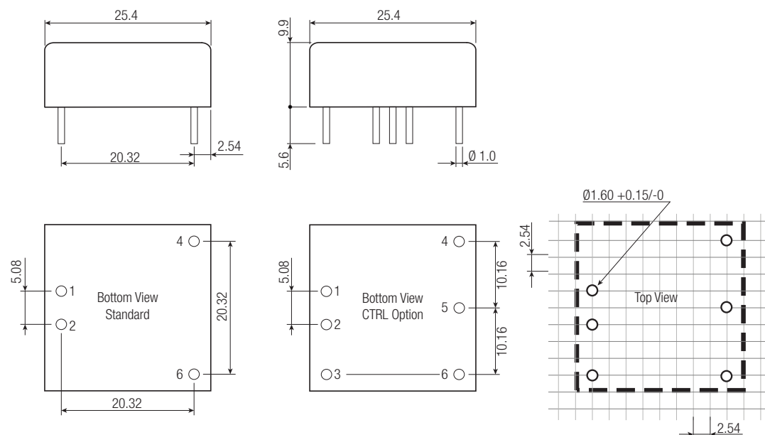
Dimension Drawing (mm)
