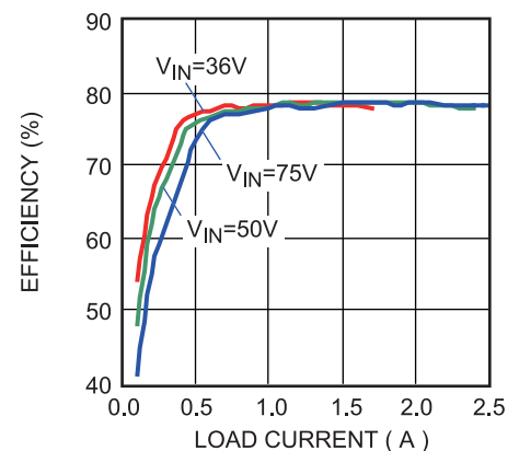
Load Efficiency
