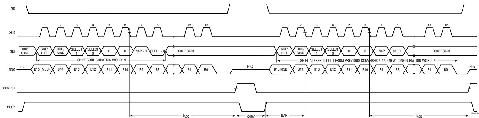
Figure 9. Nap Mode Operation for the LTC1856*
