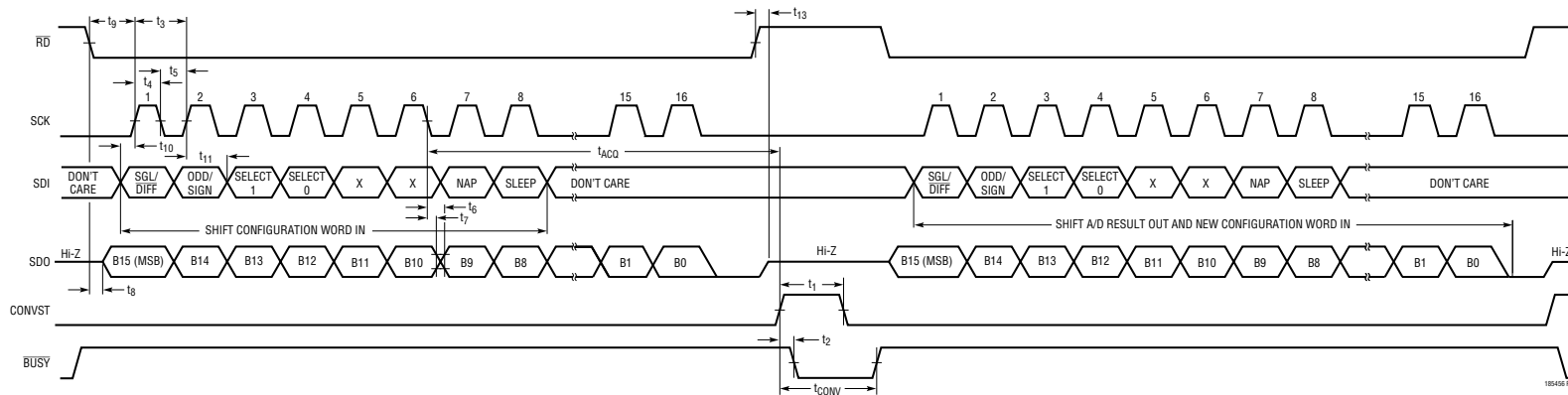
Figure 7. Operating Sequence for the LTC1856*
