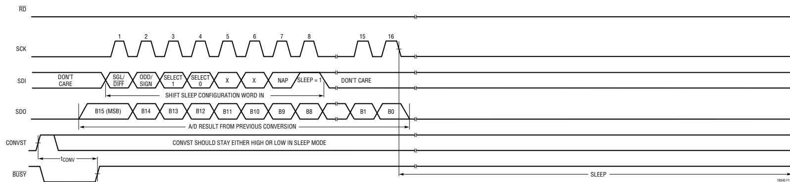
Figure 10. Sleep Mode Operation for the LTC1856*
