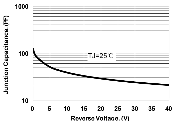
Fig.1-Typical Junction Capacitance
