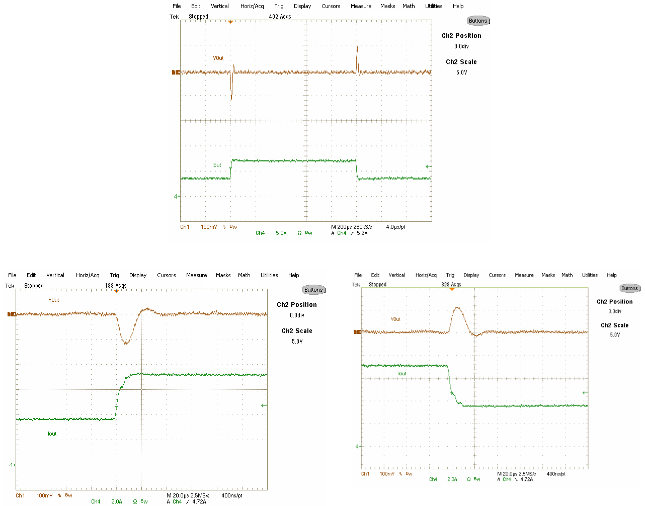
Fig. 13: Transient Response, 3.5A to 7A step
