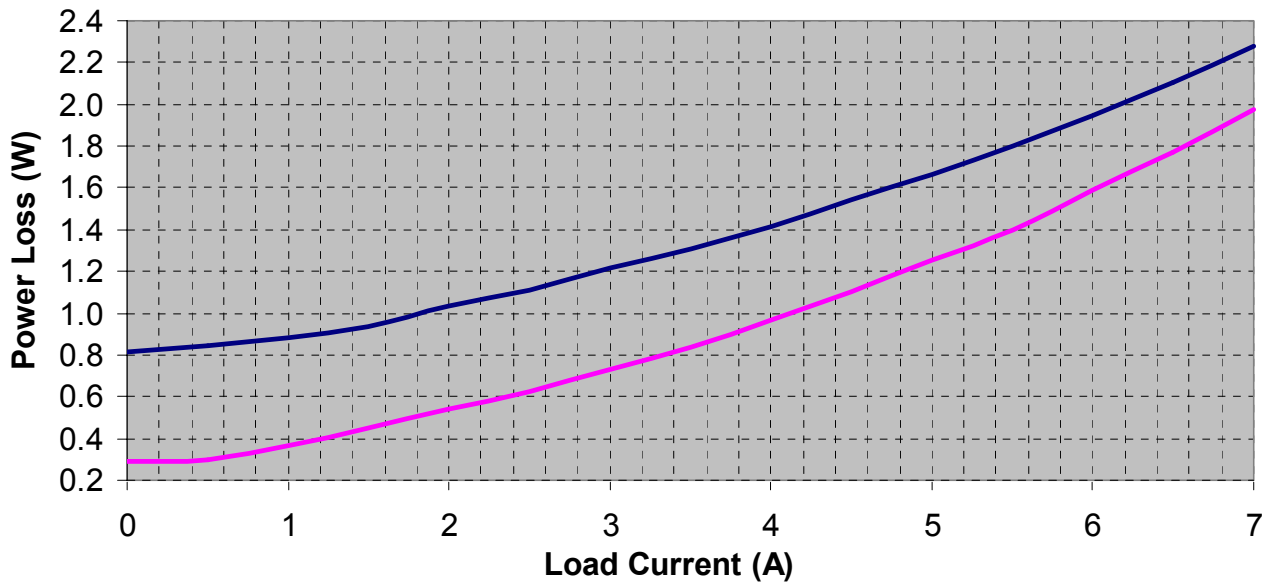
Fig.15: Efficiency versus load current
