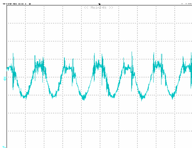
Figure 14: Output voltage ripple at nominal input voltage and rated load current ( I_o=25\text{A} )(20 mV/div, 2us/div) Load capacitance: 1\mu\text{F} ceramic capacitor and 10\mu\text{F} tantalum capacitor. Bandwidth: 20 MHz.
