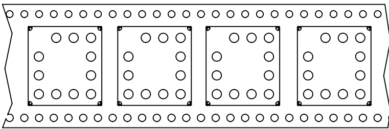
CARRIER TAPE
