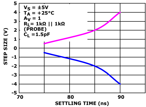
FIGURE 28. STEP SIZE vs SETTLE TIME
