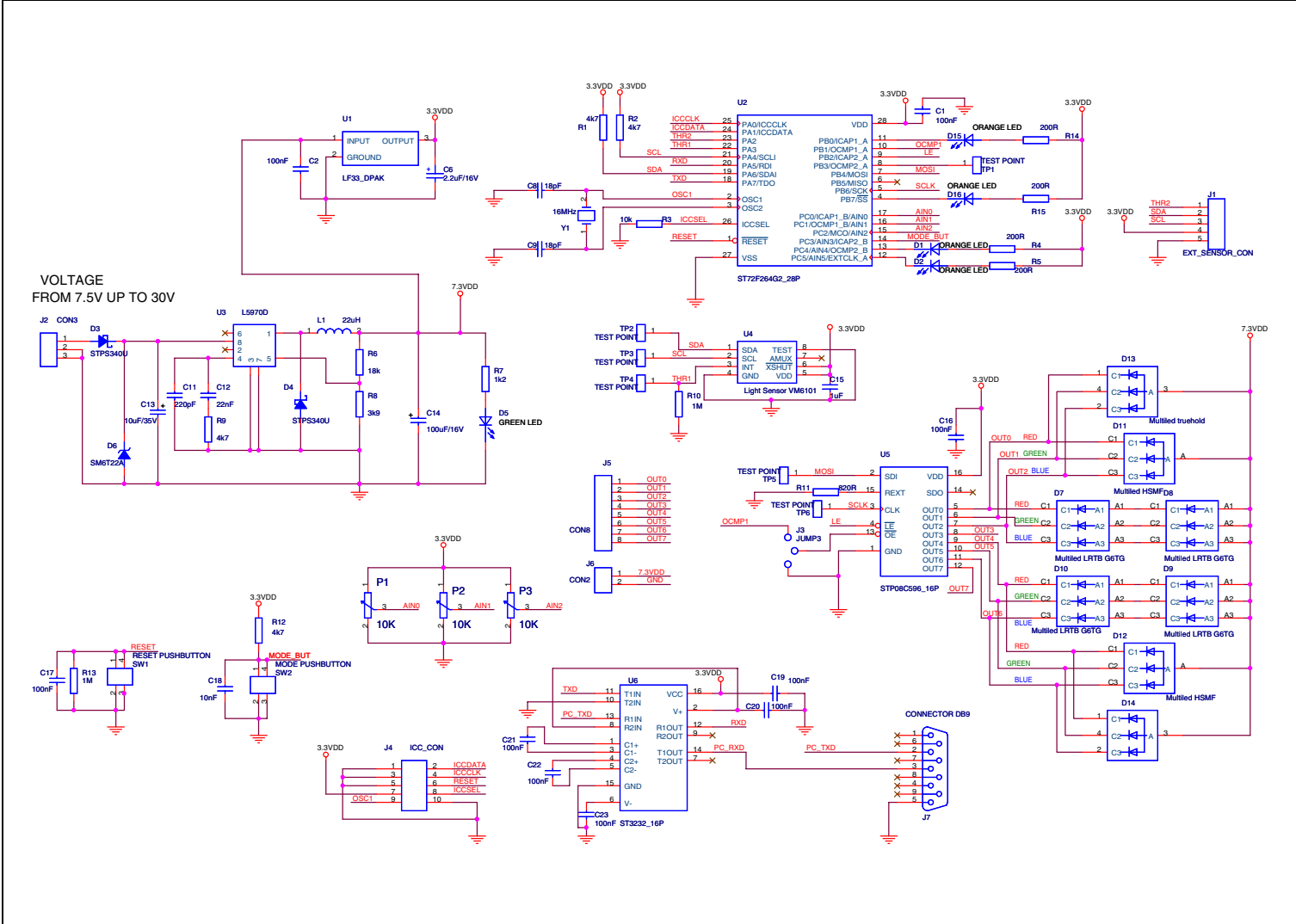
Figure 1. Schematic
