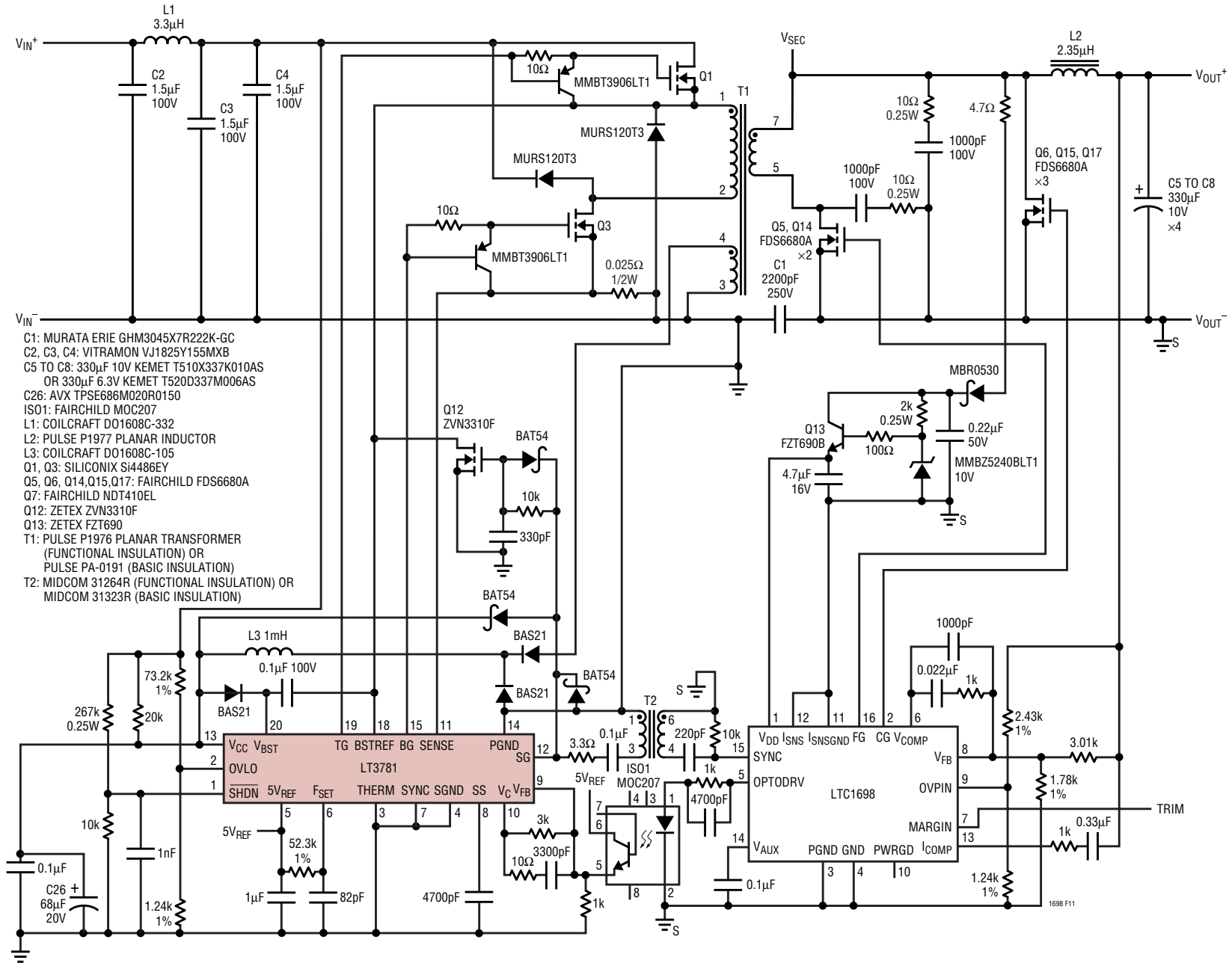
Figure 8. 36V to 72V DC in to 3.3V/20A Isolated Synchronous Forward Converter
