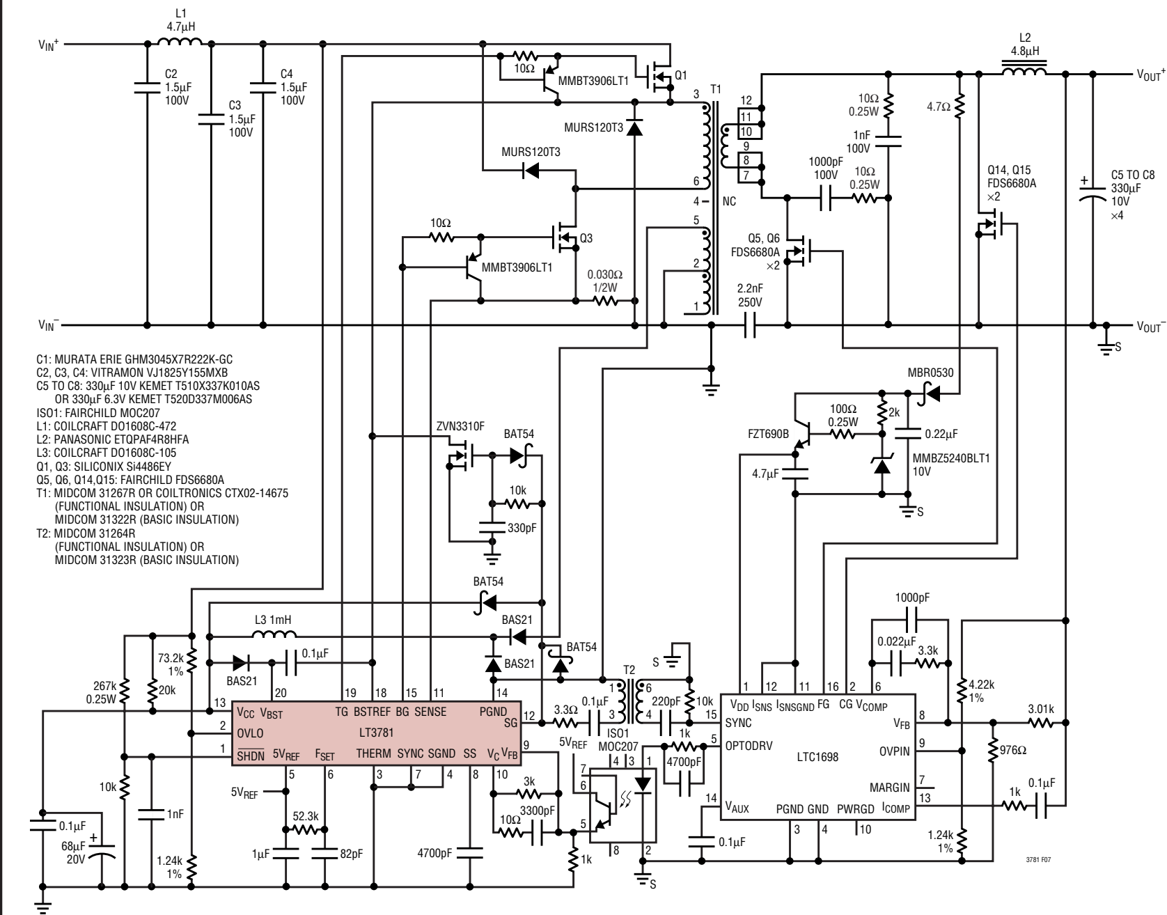
Figure 7. 36V to 72V DC in to 5V/10A Isolated Synchronous Forward Converter
