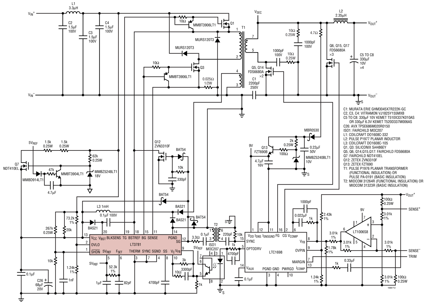
Figure 9. 36V to 72V DC in to 3.3V/20A Isolated Synchronous Forward Converter with Fast Start and Differential Sense
