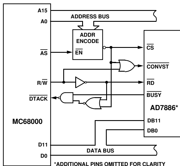
Figure 20. AD7886–MC68000 Interface
