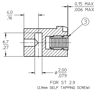
SECTION Y-Y
