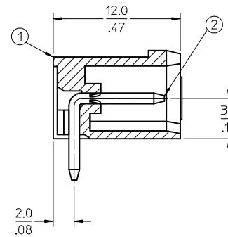
SECTION Z-Z
