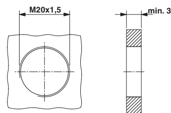
Dimensioned drawing
