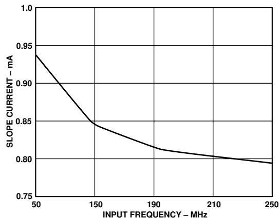
Figure 14. Slope Current, I_T , vs. Input Frequency
