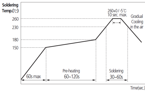
REFLOW SOLDERING
