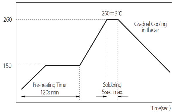
FLOW SOLDERING
