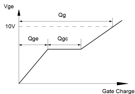
Gate Charge
