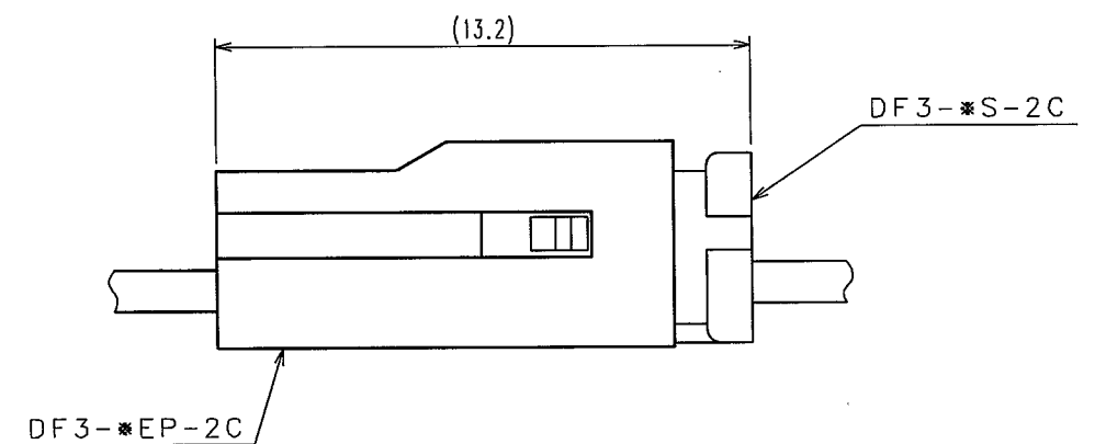
MATED CONNECTORS
