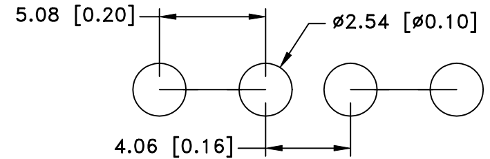
MOUNTING DETAIL
